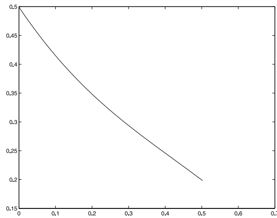
Fig. 2. Effective compliance S^e as a function of area fraction \theta .
